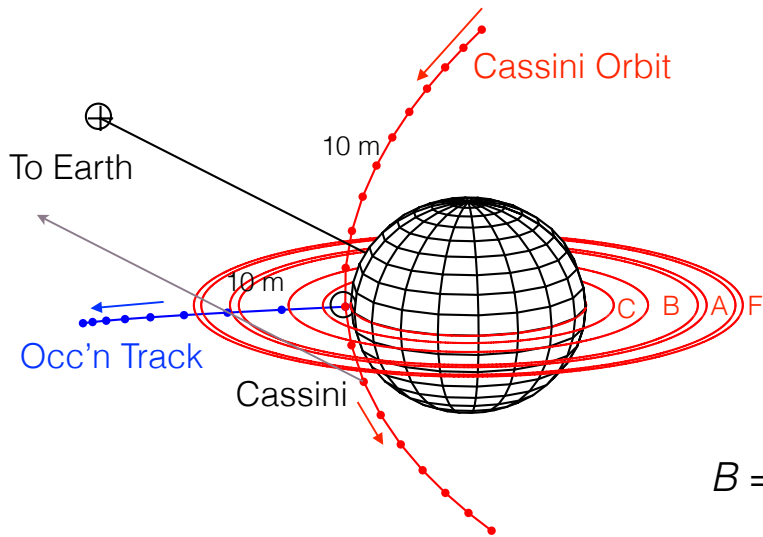
Close (Periapse) Ring Occultation Side View
