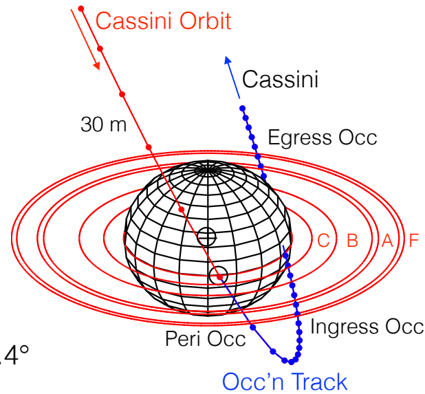
Distant Ring Occultations View from the Earth
